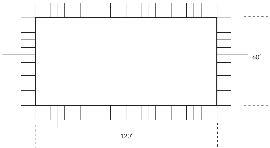
Stake Line Tie Out
